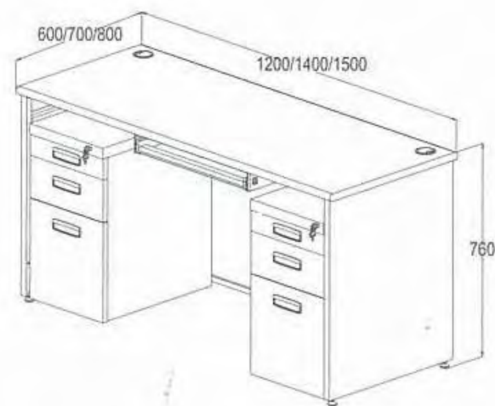
CW118-1260/DP 體積 Size: W1200*D600*H760mm CW118-1270/DP 體積 Size: W1200*D700*H760mm CW118-1470/DP 體積 Size: W1400*D700*H760mm CW118-1580/DP 體積 Size: W1500*D800*H760mm
