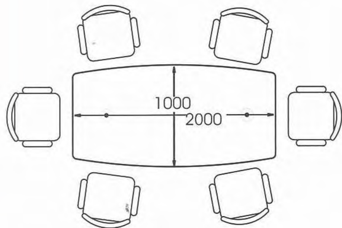
CW-CFA2010 體積Size:W2000 D1000 H750 mm
