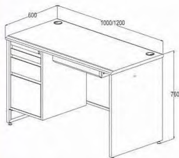
NY-1060/LP 體積Size: W1000*D600*H760mm NY-1260/LP 體積Size: W1200*D600*H760mm
