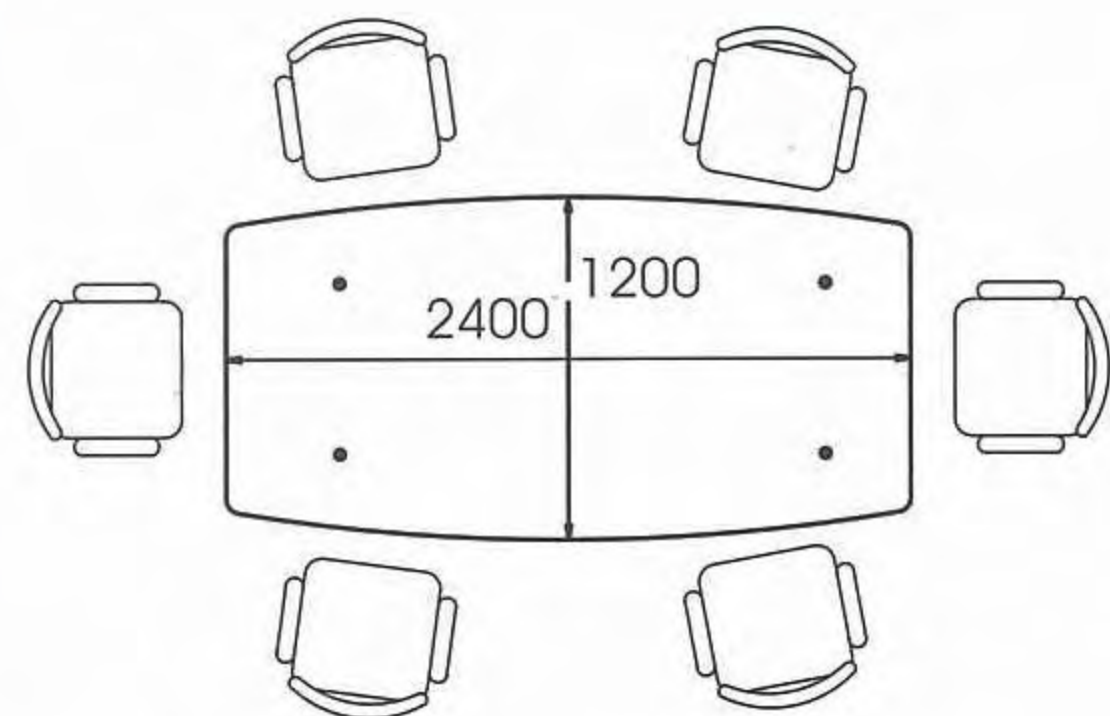
CW-CFB2412 體積Size:W2400 D1200 H750 mm
